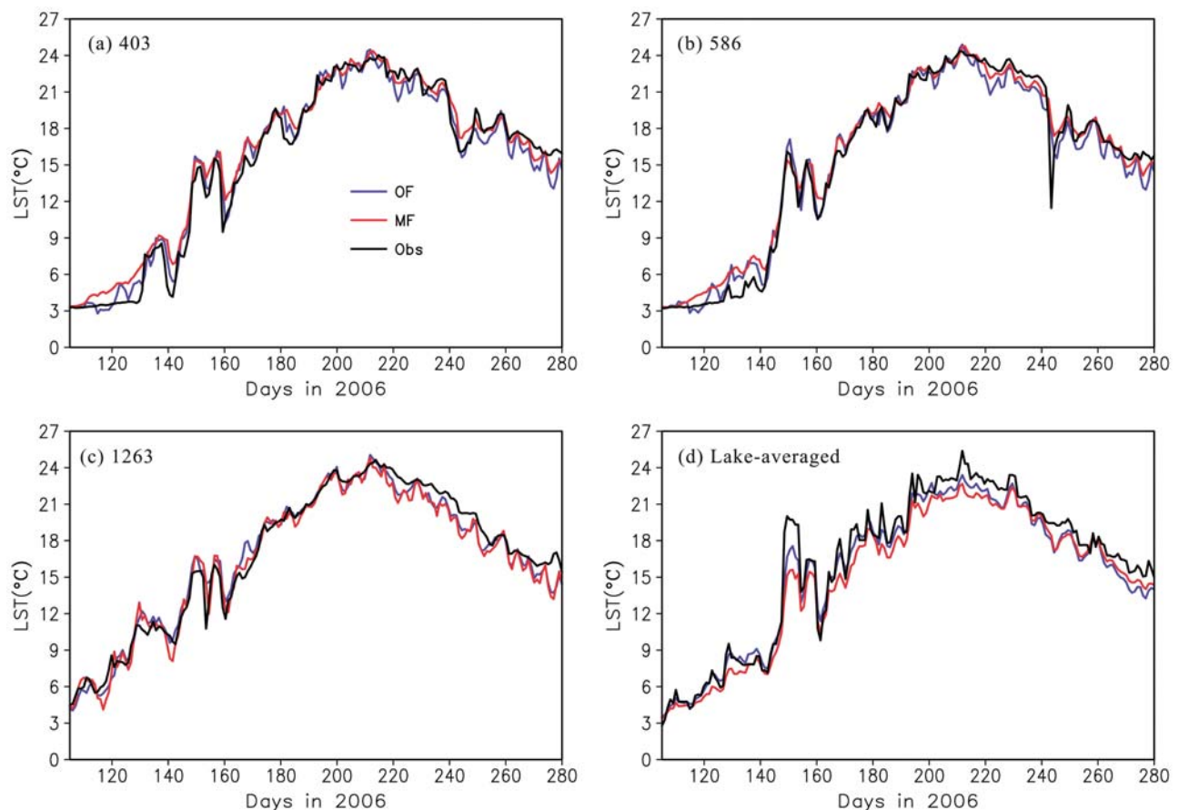
Figure 3. Time series of the observed and modeled lake surface temperature at stations (a) 403, (b) 586, (c) 1263 and (d) averaged over the whole lake.
