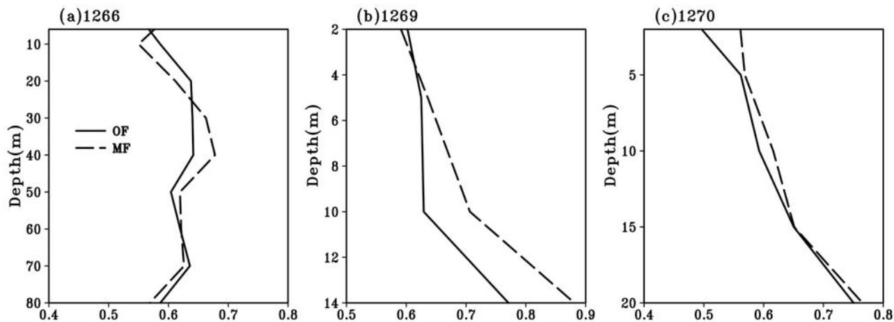
Figure 6. The vertical profile of normalized Fourier norms between simulated and observed currents at stations (a) 1266, (b) 1269, and (c) 1270.
